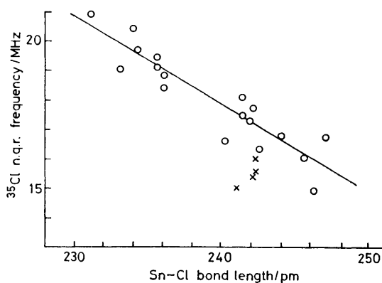
FIGURE 3 Sn-Cl bond length correlation with 35 Cl n.q.r. frequency, SnCl 4 ·2L (O) and M 2 [SnCl 6 ] (×)
